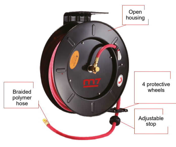
SA4320A PNEUMATIC HOSE REEL
